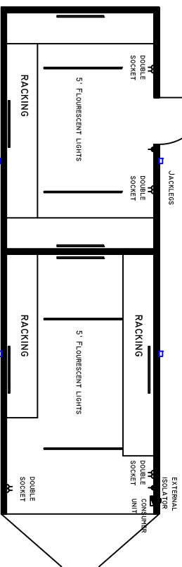
32' x 10' Split Stores Unit
