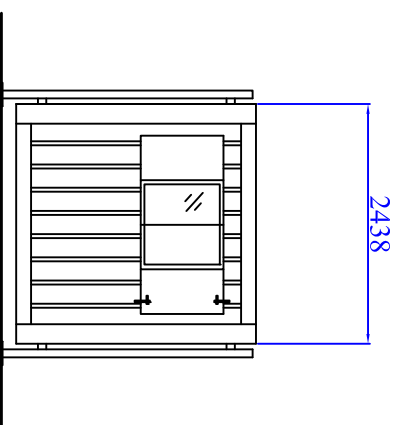
SIDE ELEVATION
